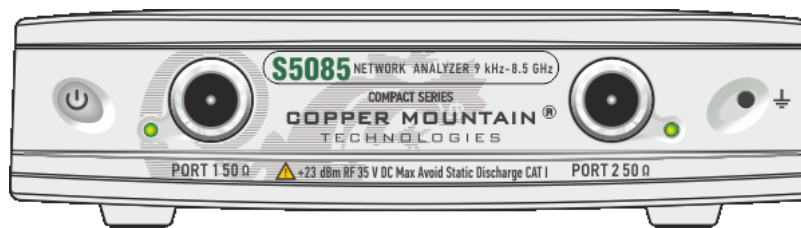
S5085 front panel
