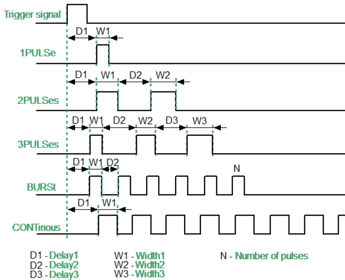
Pulse generator timing diagram
