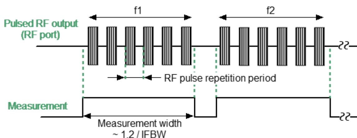
Asynchronous pulse
